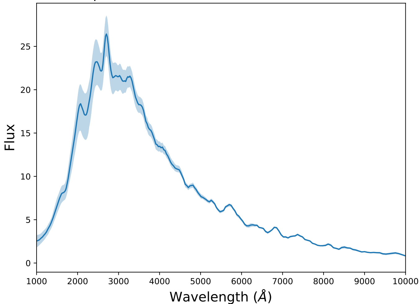
Spectrum 9 for transient CCSN at z=0.99
